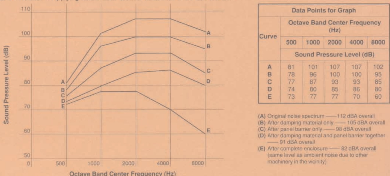
Figure 1 Results of Applying Basic Noise Control Measures to a Parts Tumbler
