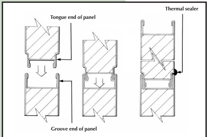
Figure 2—Assembly oven panel
