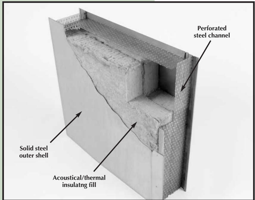
Figure 1—Oven panel construction
