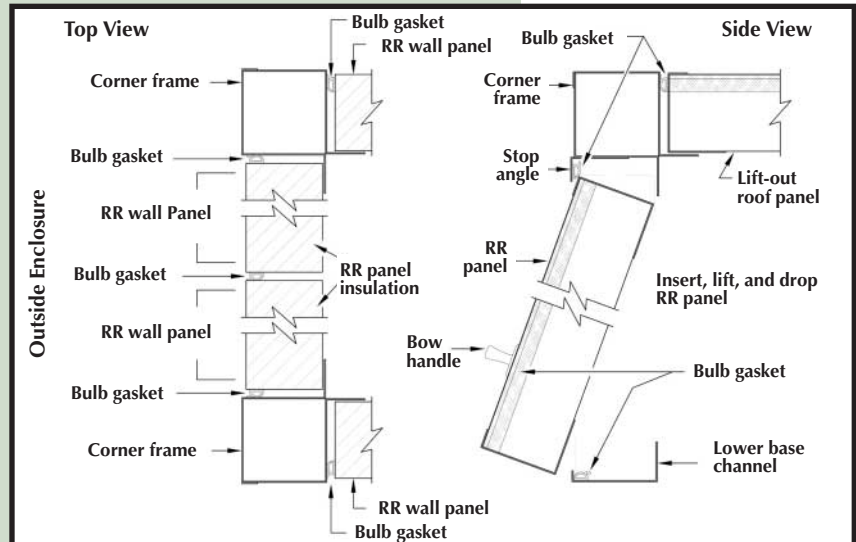
Figure 3—Assembly of Type RR panels
