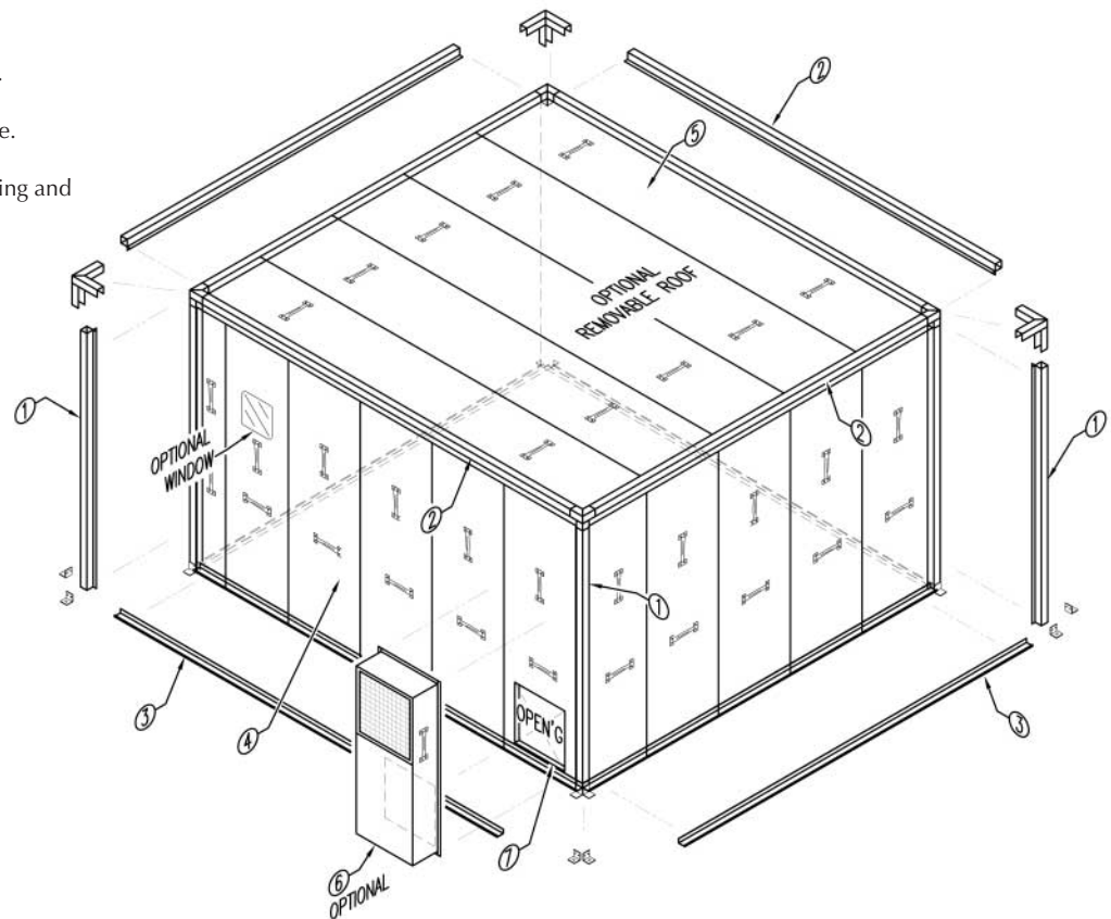
Figure 1—Assembly of typical Type RR acoustical enclosure
