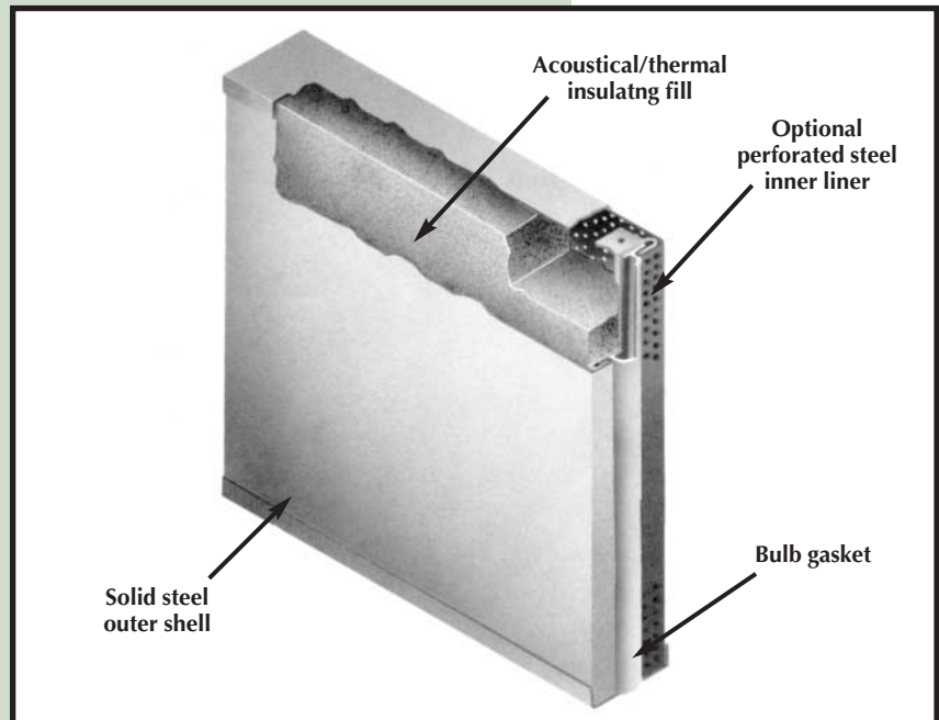
Figure 2—Standard Type RR panel construction
